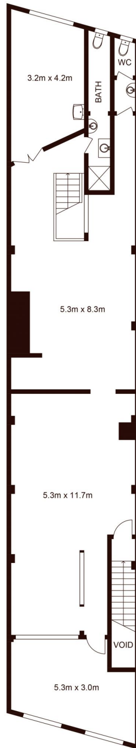
FIRST FLOOR
